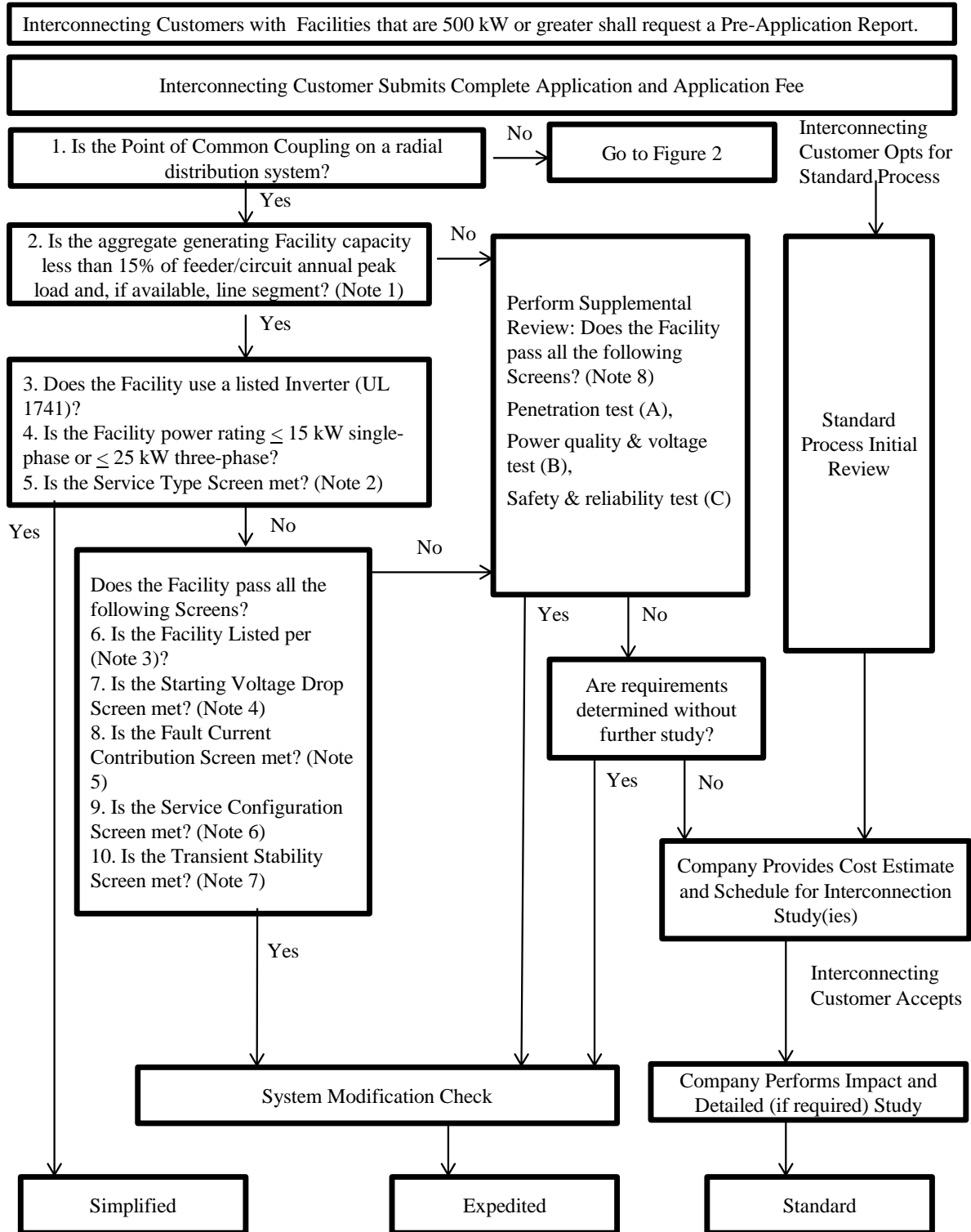
Figure 1 – Schematic of Massachusetts DG Interconnection Process
